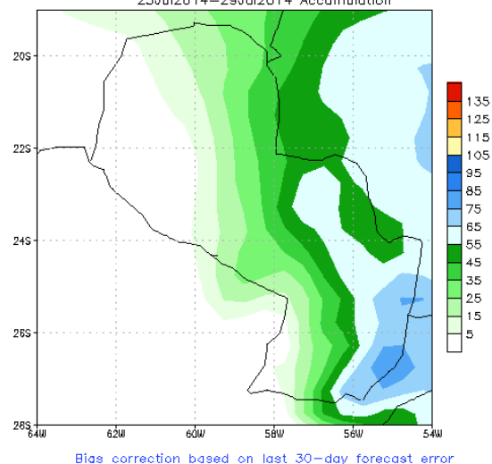
NCEP GFS Ensemble Forecast 1-7 Day Precipitation (mm) from: 23Jul2014 23Jul2014-29Jul2014 Accumulation
