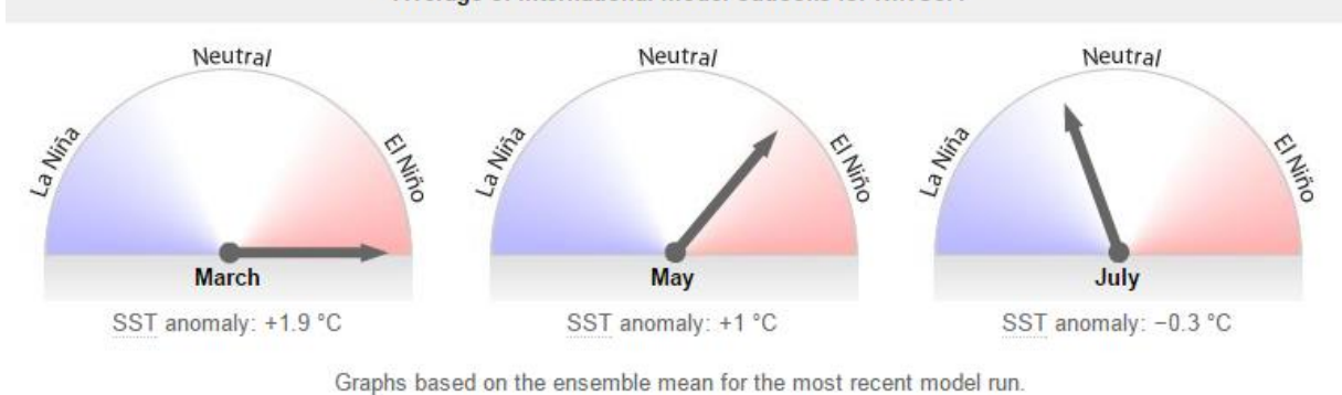
Average of international model outlooks for NINO3.4
