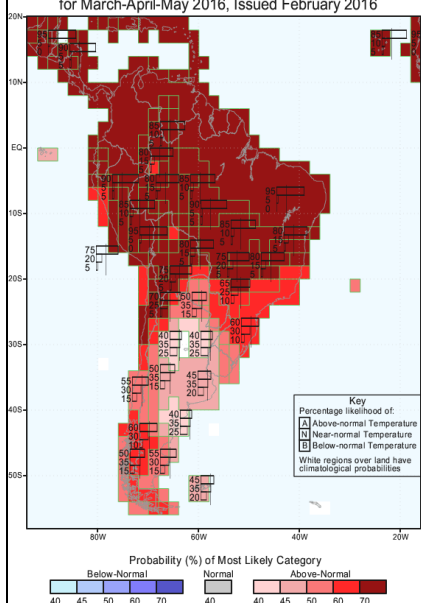
IRI Multi-Model Probability Forecast for Temperature for March-April-May 2016, Issued February 2016
