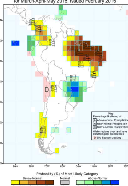
IRI Multi-Model Probability Forecast for Precipitation for March-April-May 2016, Issued February 2016
