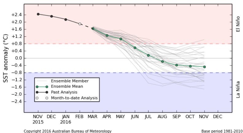
POAMA monthly mean NINO34 - Forecast Start: 28 FEB 2016
