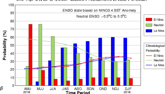
Mid-Apr IRVPC Model-Based Probabilistic ENSO Forecast
