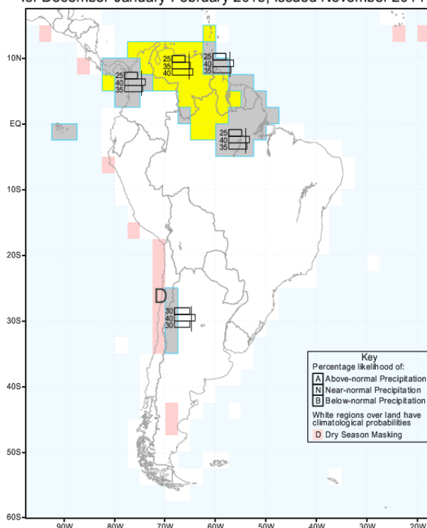
IRI Multi-Model Probability Forecast for Precipitation for December-January-February 2015, Issued November 2014
