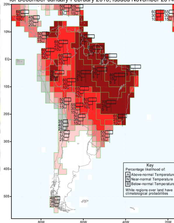
IRI Multi-Model Probability Forecast for Temperature for December-January-February 2015, Issued November 2014
