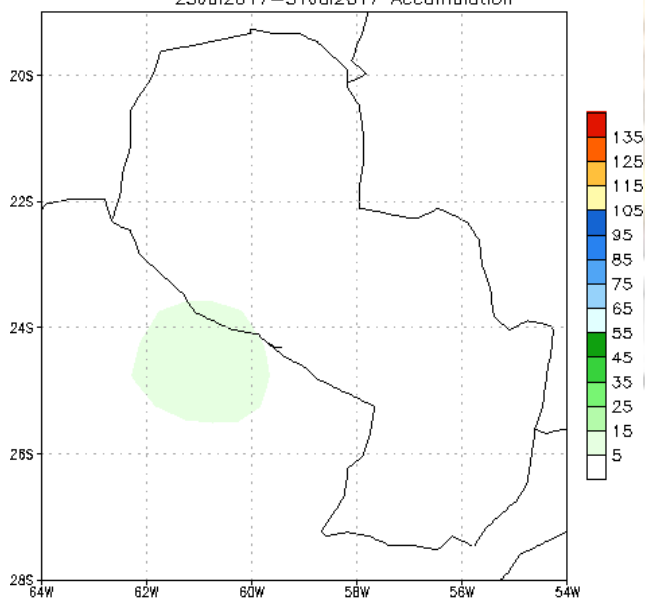
NCEP GFS Ensemble Forecast 1-7 Day Precipitation (mm) from: 25Jul2017 25Jul2017-31Jul2017 Accumulation
